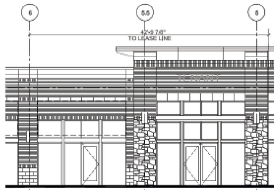
NORTH ELEVATION SCALE: 1/4"=1'-0"
