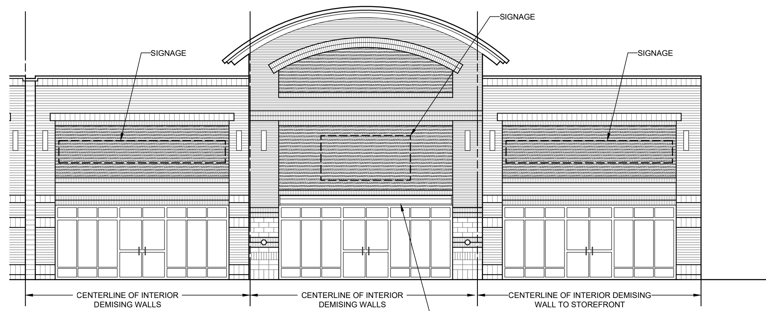
2 ELEVATIONS SCALE: 1/8"=1'-0"
