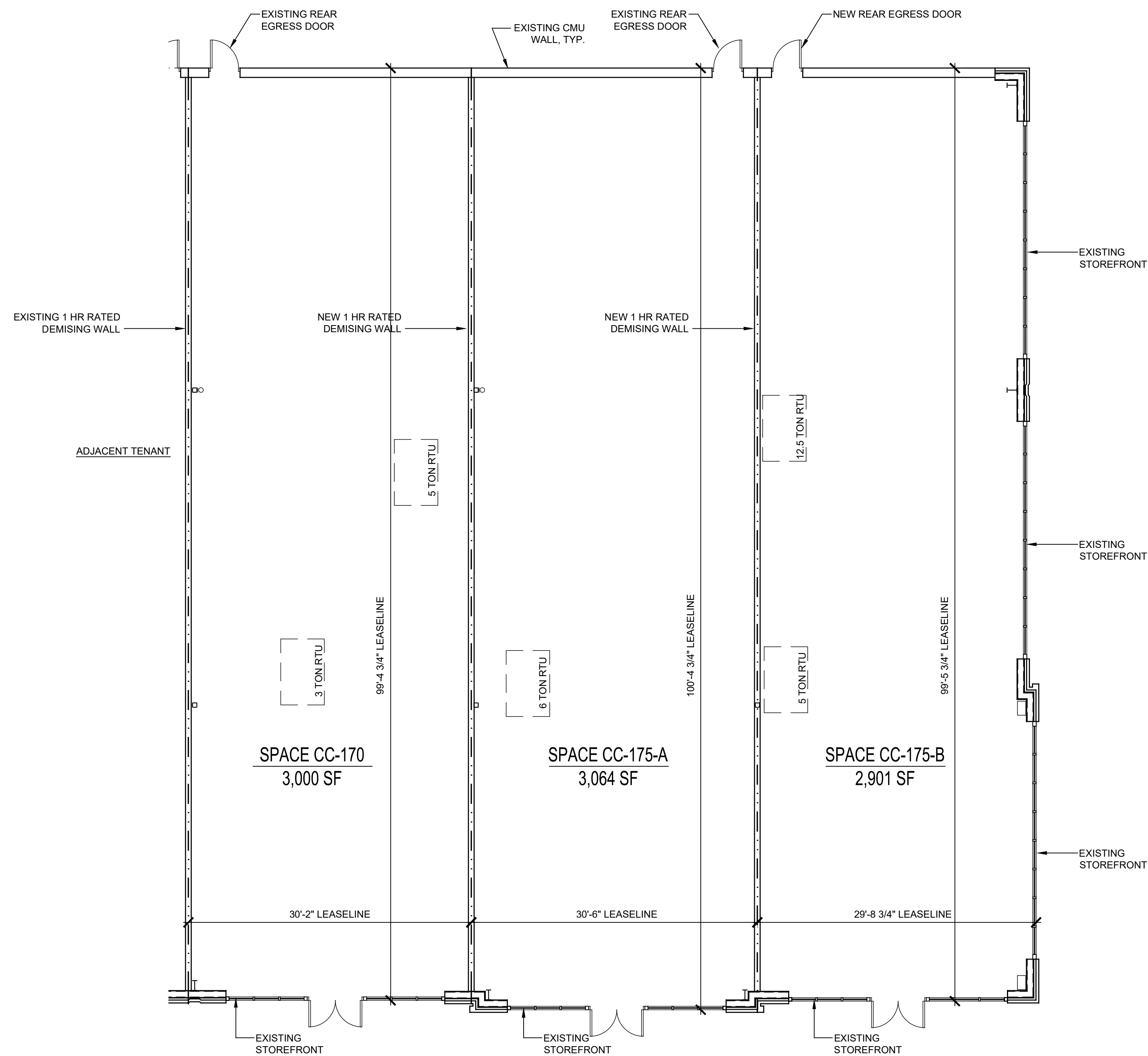
3 LEASE PLAN SCALE: 1/8"=1'-0"
